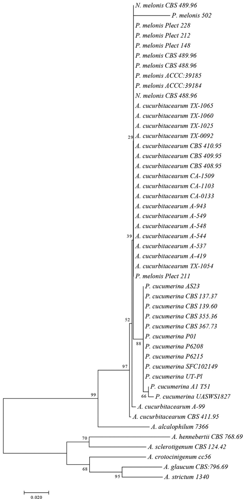
Fig. 1. The phylogenetic tree constructed by the neighbour-joining analysis of the partial 5.8S rRNA sequences of P. melonis strain 502 and references P. melonis from GenBank. The sequences of Acromonium genus fungi were accepted as an outgroup
